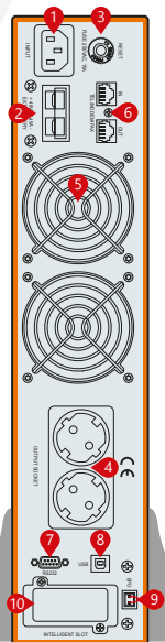
Rear Panel 2-3kVA
